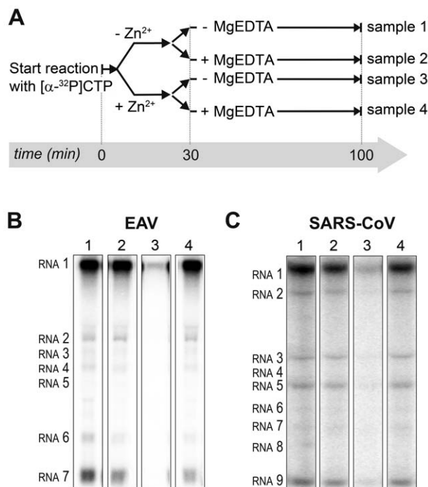
Figure 3. Inhibition of nidovirus RTC activity by Zn 2+ can be reversed by chelation. (A) Schematic representation of the in vitro assays with isolated RTCs, which were initiated with [\alpha\text{-}^{32}\text{P}]\text{CTP} , either in the absence (sample 1 and 2) or presence of 500 \mu\text{M} Zn 2+ . After a 30-min incubation at 30°C, both the untreated and Zn 2+ -treated samples were split into two aliquots, and 1 mM of the Zn 2+ chelator MgEDTA was added to samples 2 and 4. All reactions were subsequently incubated for another 70 min before termination. (B) Analysis of RNA products synthesized in assays with EAV RTCs. Numbers above the lanes refer to the sample numbers described under (A). (C) In vitro activity assay with SARS-CoV RTCs.
